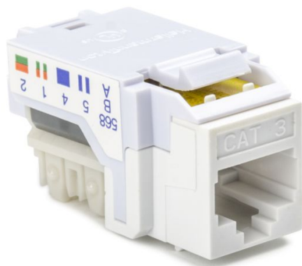
Category 3, 6P6C RJ11 USOC Keystone Jack, White, 1/bag
